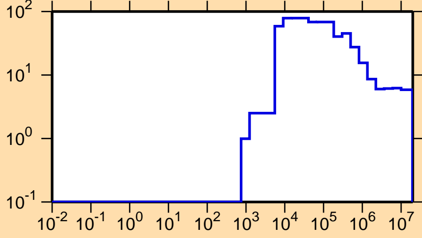
\Delta\sigma/\sigma vs. E for ^{138}\text{Xe}(n,\text{nonel.})
