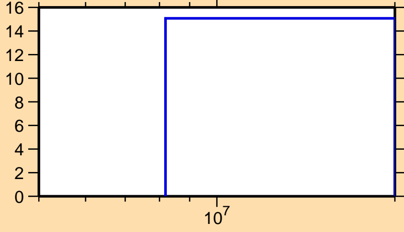
\Delta\sigma/\sigma vs. E for ^{138}\text{Xe}(n,el.)
