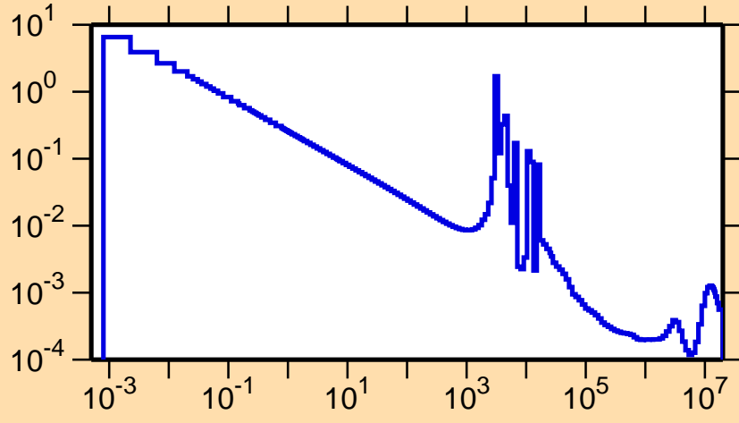
\sigma vs. E for ^{139}\text{Xe}(n,\gamma)
