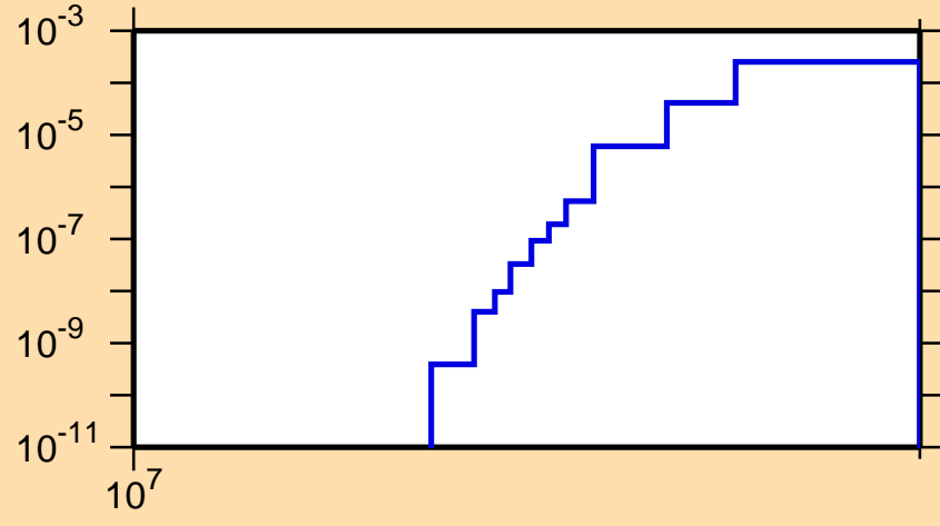
\sigma vs. E for ^{139}\text{Xe}(n,np)
