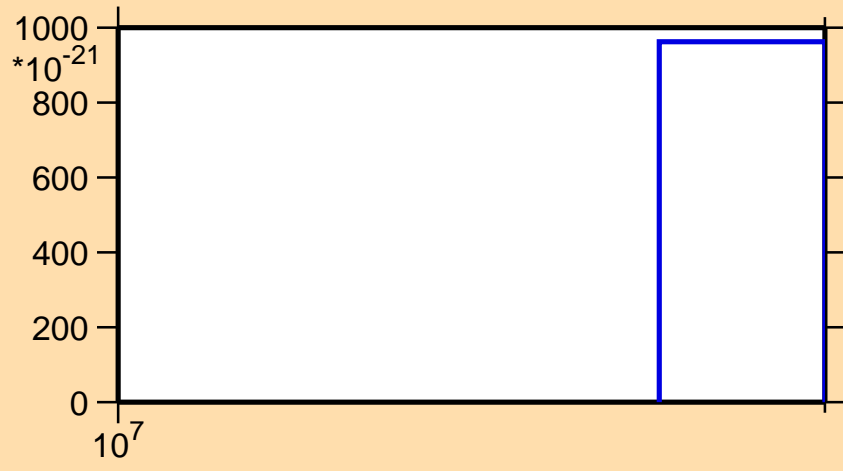
\sigma vs. E for ^{139}\text{Xe} (mt 42)
