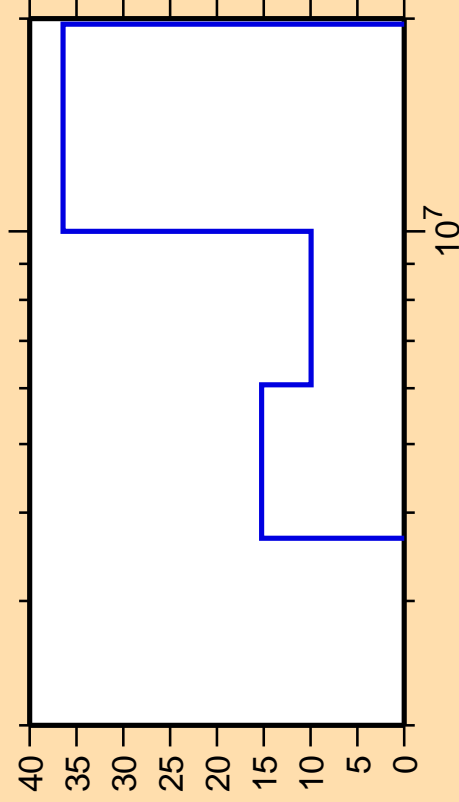
\Delta\sigma/\sigma vs. E for ^{139}\text{Xe}(n,2n)
