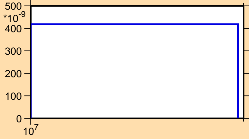
\sigma vs. E for ^{139}\text{Xe}(n,nt)
