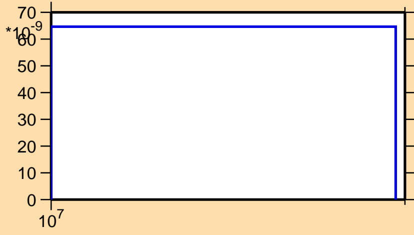
\sigma vs. E for ^{139}\text{Xe}(n,\text{nd})
