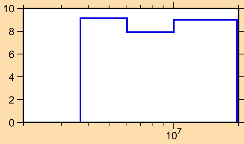
\Delta\sigma/\sigma vs. E for ^{139}\text{Xe}(n,\text{nonel.})
