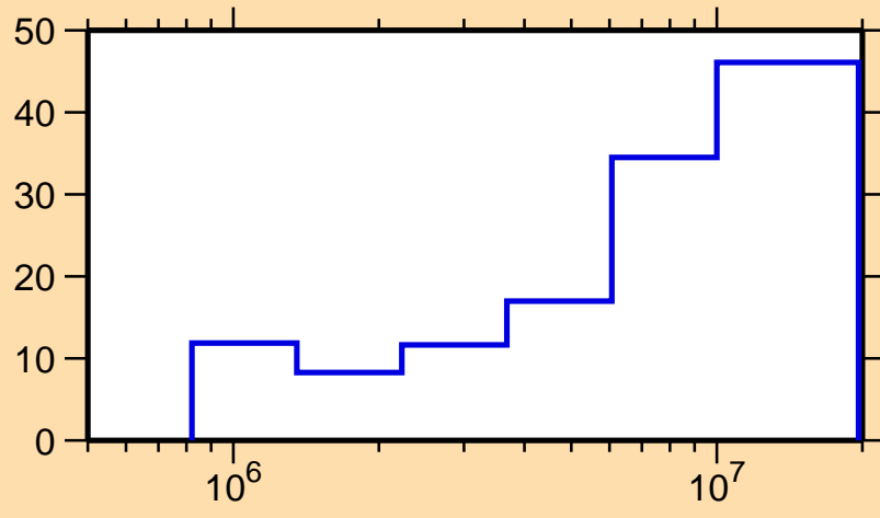
\Delta\sigma/\sigma vs. E for ^{139}\text{Xe}(n,\text{inel.})
