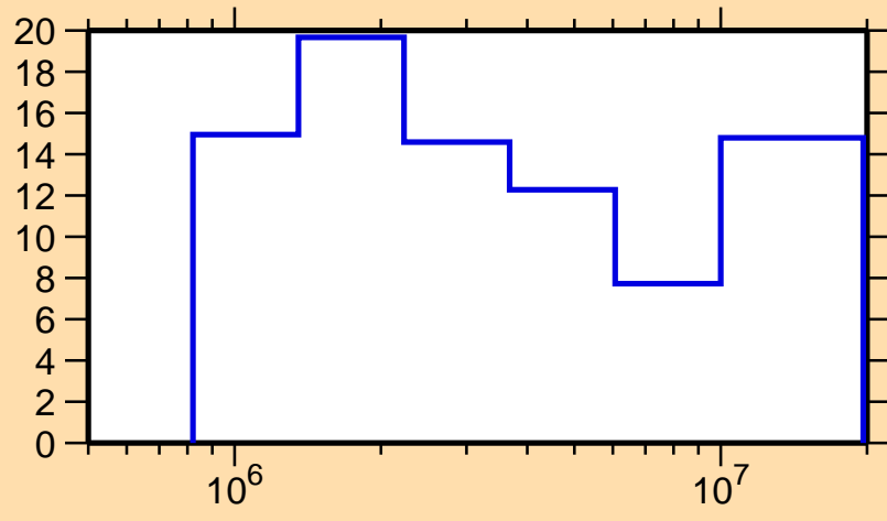
\Delta\sigma/\sigma vs. E for ^{139}\text{Xe}(n,\text{tot.})
