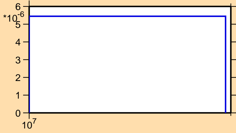
\sigma vs. E for ^{139}\text{Xe}(n,np)
