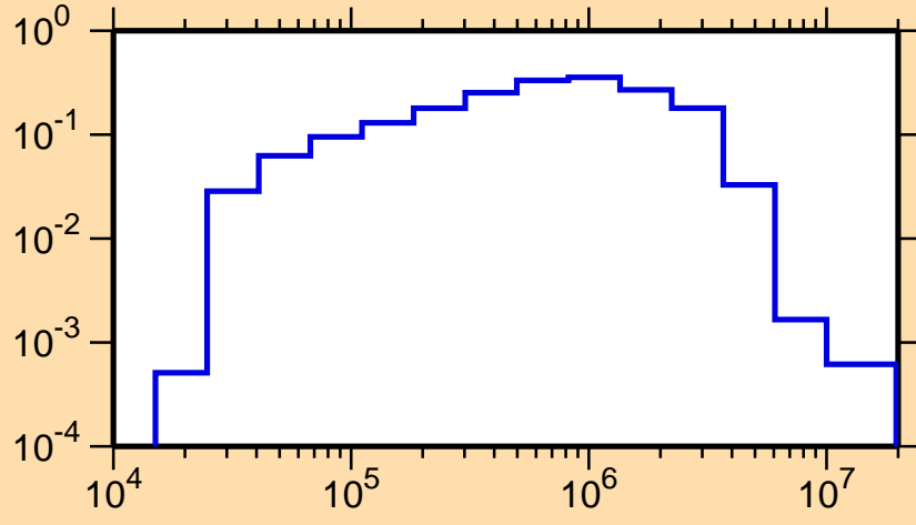
\sigma vs. E for ^{139}\text{Xe}(n,n_1)
