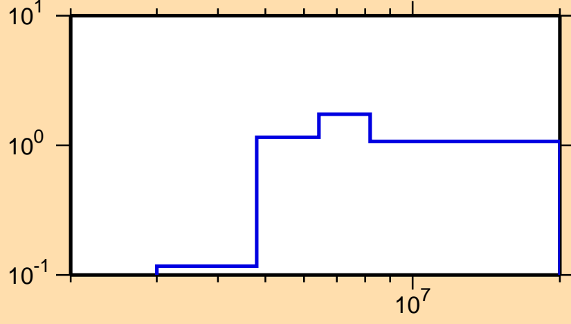
\sigma vs. E for ^{139}\text{Xe}(n,2n)
