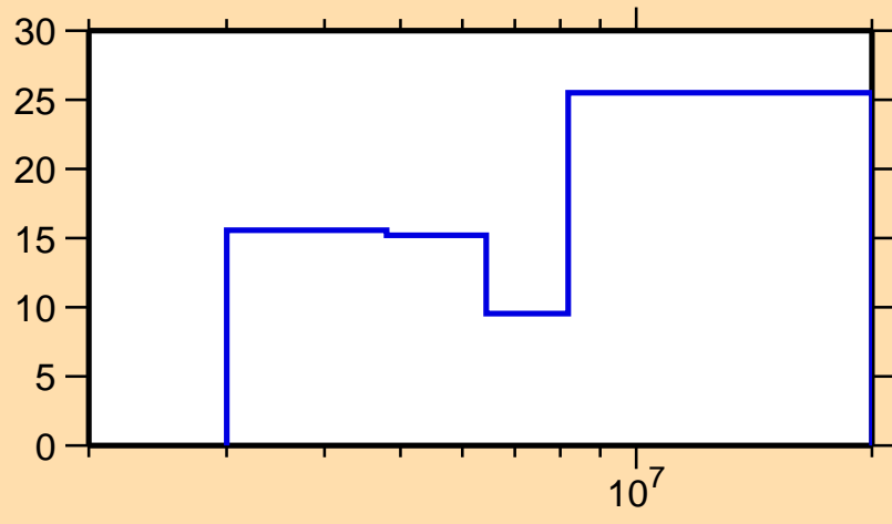
\Delta\sigma/\sigma vs. E for ^{139}\text{Xe}(n,2n)
