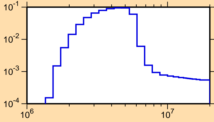
\sigma vs. E for ^{140}\text{Xe}(n,n_4)
