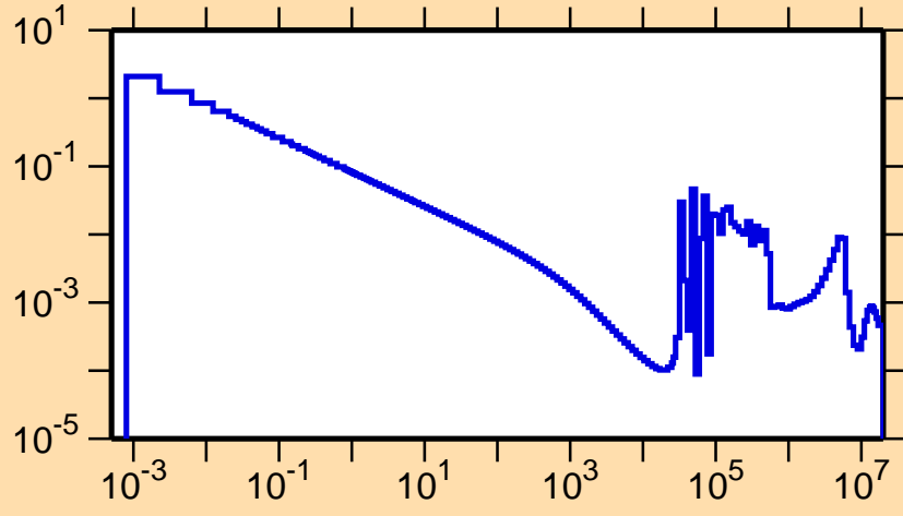
\sigma vs. E for ^{140}\text{Xe}(n,\gamma)
