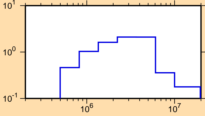
\sigma vs. E for ^{140}\text{Xe}(n,\text{inel.})
