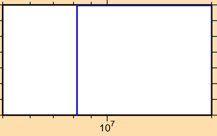
\sigma vs. E for ^{140}\text{Xe}(n,nt)
