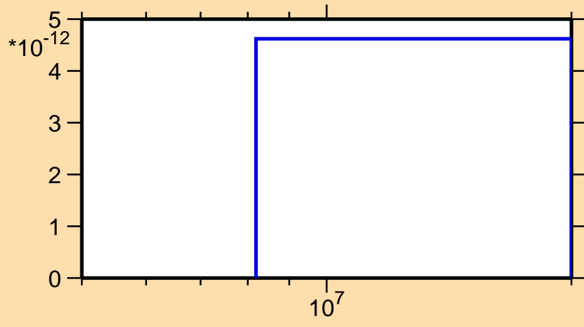
\sigma vs. E for ^{140}\text{Xe}(n,3n\alpha)
