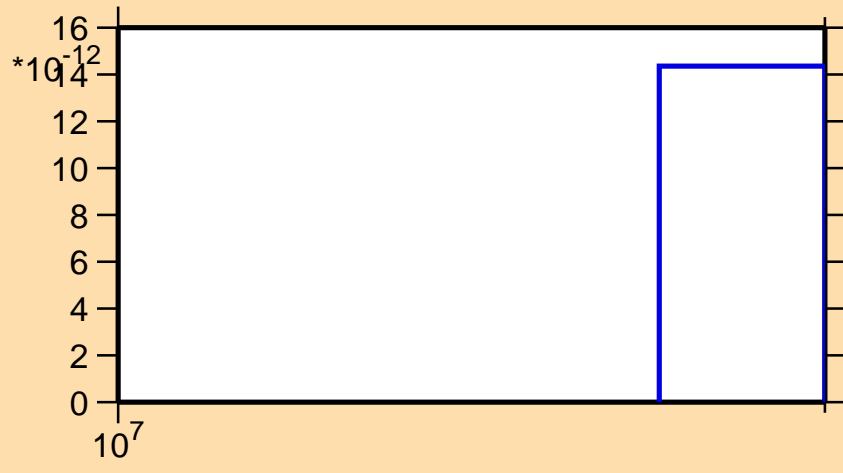
\sigma vs. E for ^{142}\text{Xe}(n,2np)
