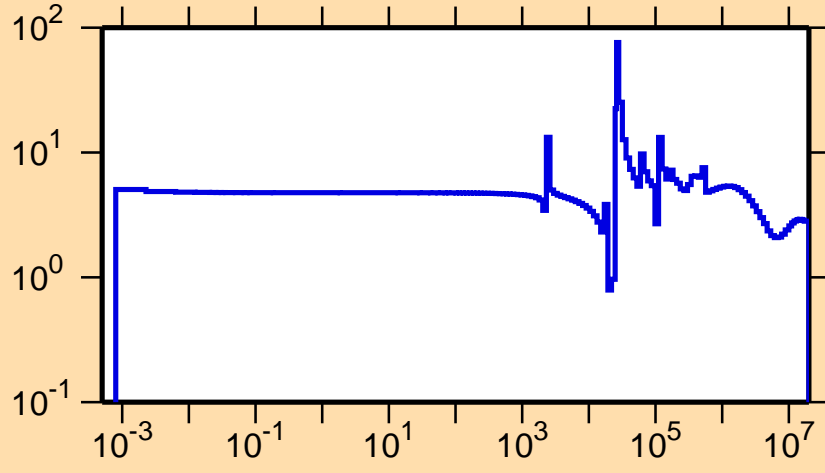
\sigma vs. E for ^{142}\text{Xe}(n,\text{el.})
