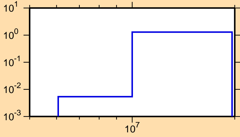
\sigma vs. E for ^{142}\text{Xe}(n,3n)
