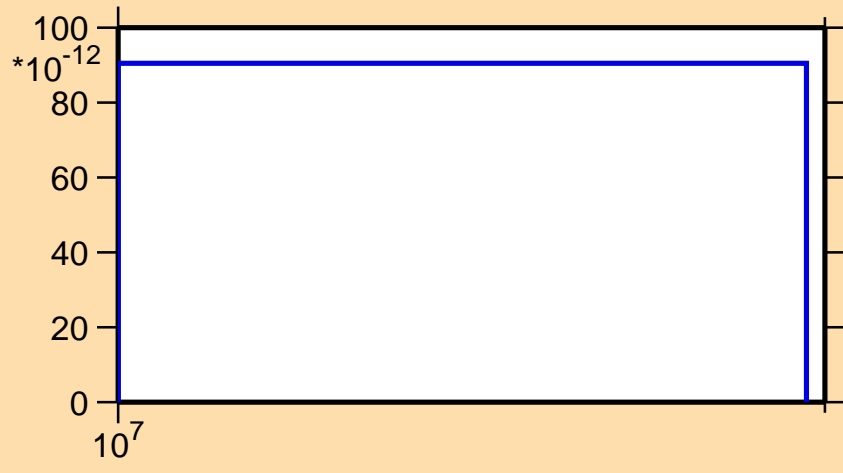
\sigma vs. E for ^{142}\text{Xe}(n,\text{nd})
