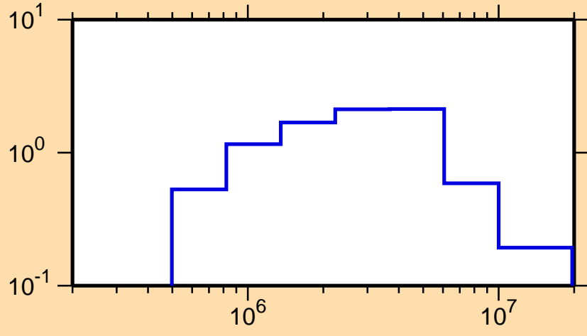
\sigma vs. E for ^{142}\text{Xe}(n,\text{inel.})
