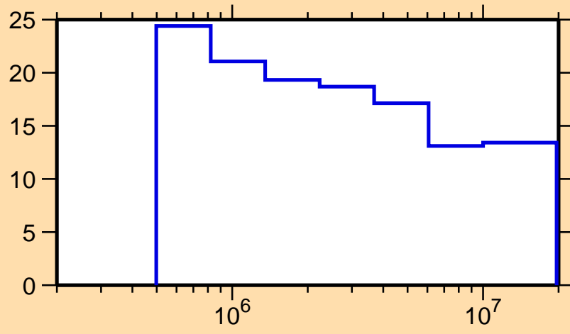
\Delta\sigma/\sigma vs. E for ^{142}\text{Xe}(n,\text{nonel.})
