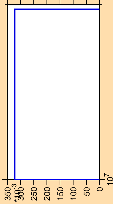
\Delta\sigma/\sigma vs. E for ^{142}\text{Xe}(n,2np)
