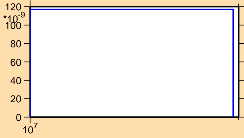
\sigma vs. E for ^{142}\text{Xe}(n,nt)
