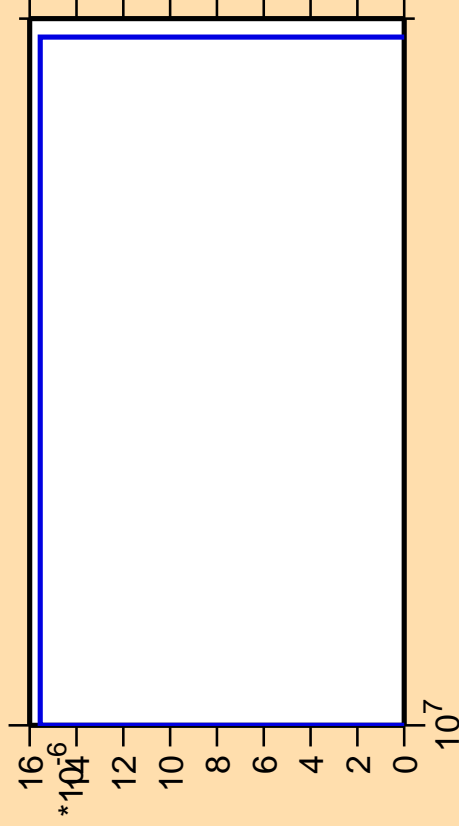
\Delta\sigma/\sigma vs. E for ^{142}\text{Xe} (mt 11)
