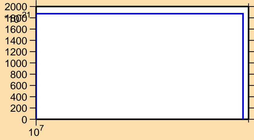
\sigma vs. E for ^{142}\text{Xe} (mt 11)
