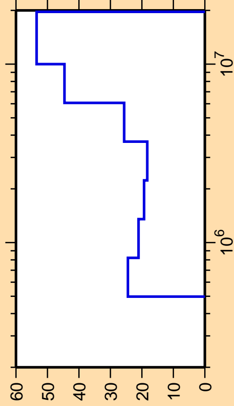
\Delta\sigma/\sigma vs. E for ^{142}\text{Xe}(n,\text{inel.})
