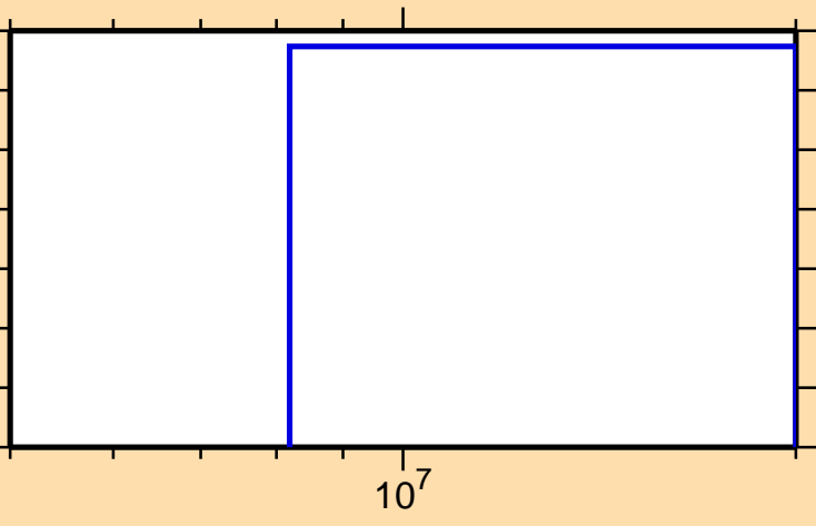
\sigma vs. E for ^{142}\text{Xe}(n,t)
