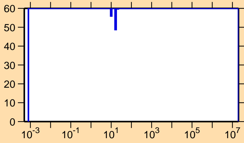
\Delta\sigma/\sigma vs. E for ^{78}\text{Y}(n,\gamma)
