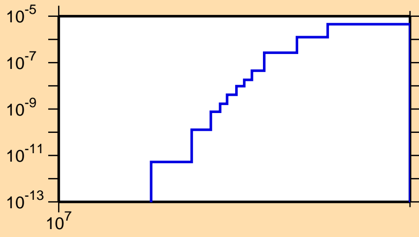
\sigma vs. E for ^{78}\text{Y}(n,\text{nd})
