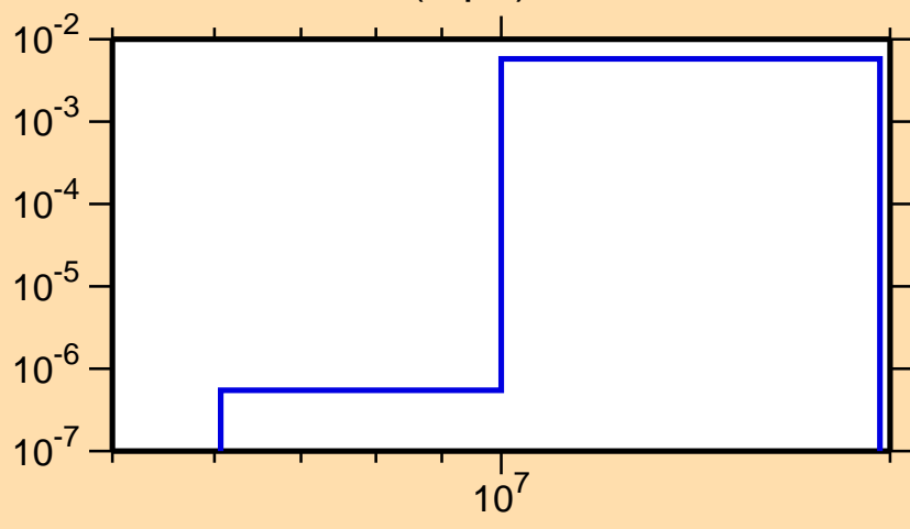
\sigma vs. E for ^{78}\text{Y}(n,\text{pd})
