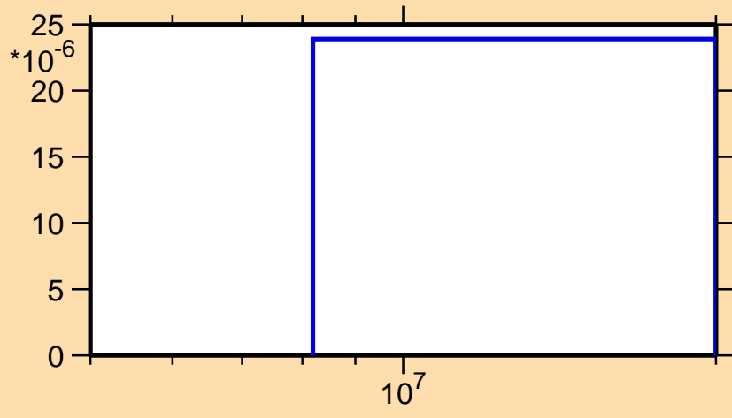
\sigma vs. E for ^{78}\text{Y}(n,\text{pt})
