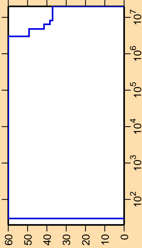
\Delta\sigma/\sigma vs. E for ^{78}\text{Y}(n,\text{inel.})
