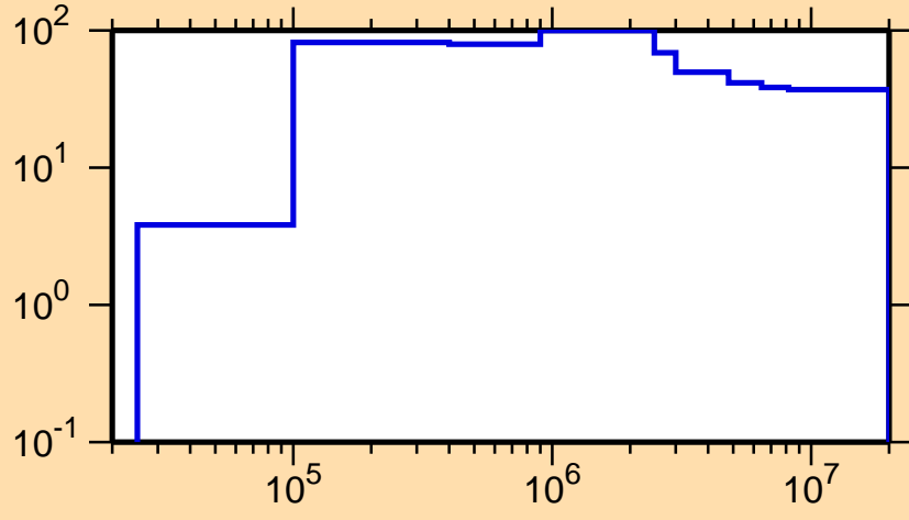
\Delta\sigma/\sigma vs. E for ^{78}\text{Y}(n,n\text{cont.})
