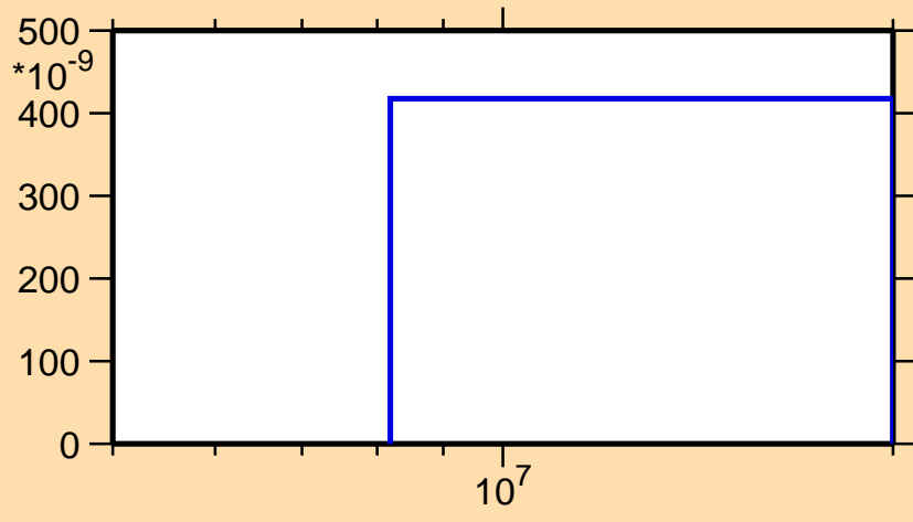
\sigma vs. E for ^{78}\text{Y}(n,2np)
