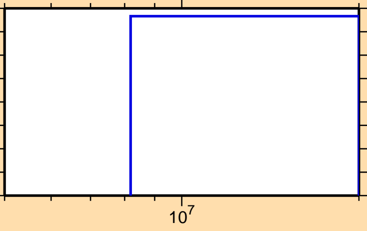
\sigma vs. E for ^{78}\text{Y}(n,2n)
