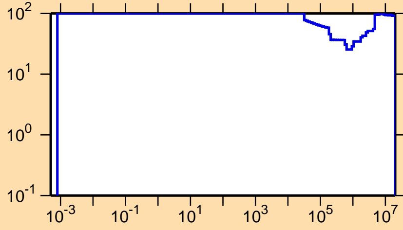
\Delta\sigma/\sigma vs. E for ^{79}\text{Y}(n,p)
