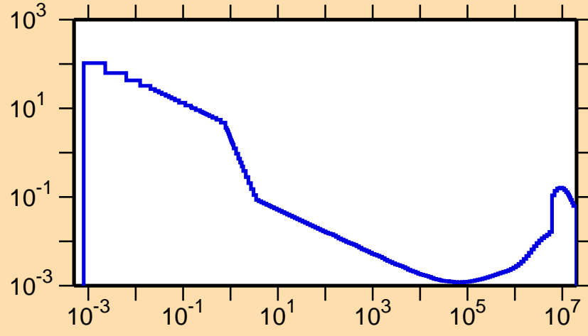
\sigma vs. E for ^{79}\text{Y}(n,\alpha)
