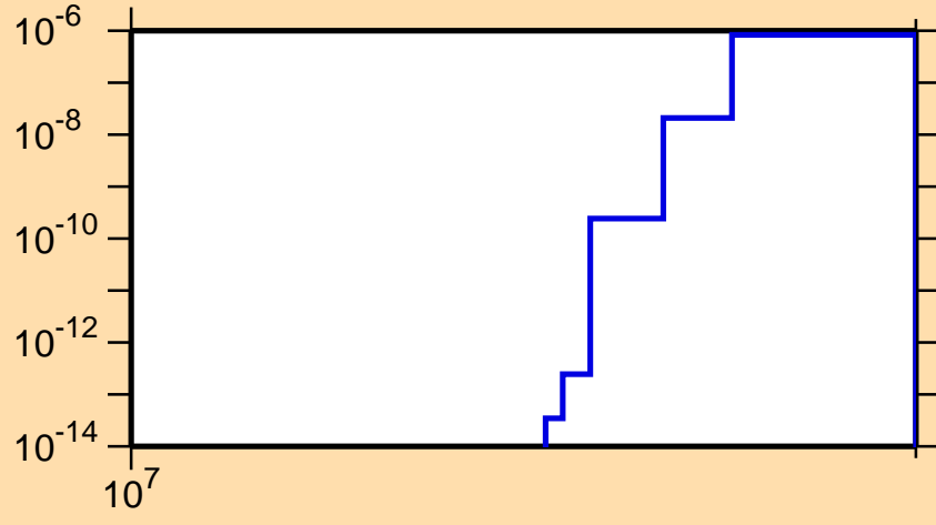
\sigma vs. E for ^{79}\text{Y}(n,\text{nd})
