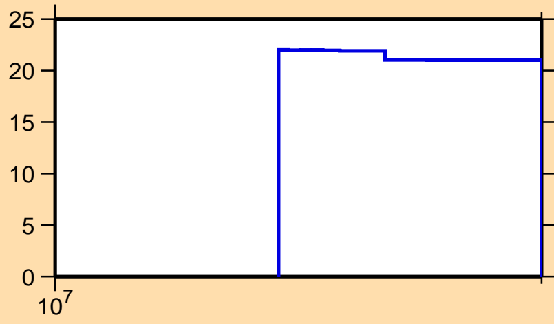
\Delta\sigma/\sigma vs. E for ^{79}\text{Y}(n,\text{tot.})
