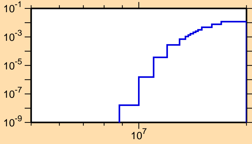
\sigma vs. E for ^{79}\text{Y}(n,pd)
