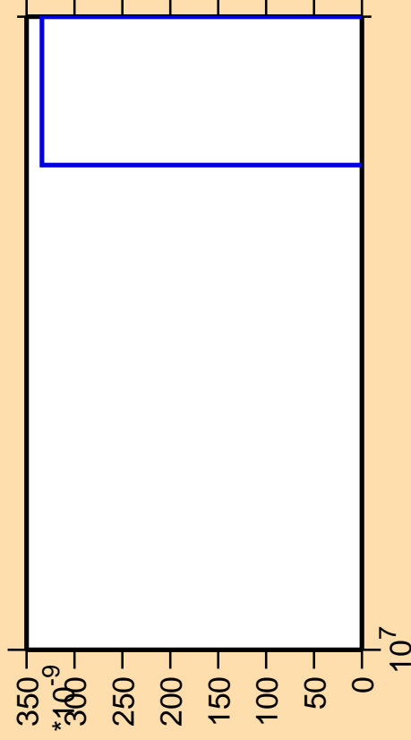
\Delta\sigma/\sigma vs. E for ^{79}\text{Y}(n,nt)
