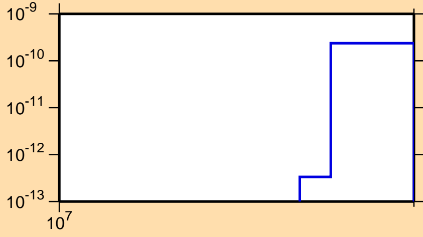
\sigma vs. E for ^{79}\text{Y} (mt 34)
