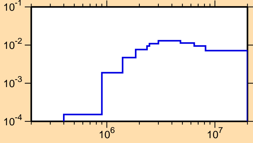
\sigma vs. E for ^{79}\text{Y}(n,n\text{cont.})
