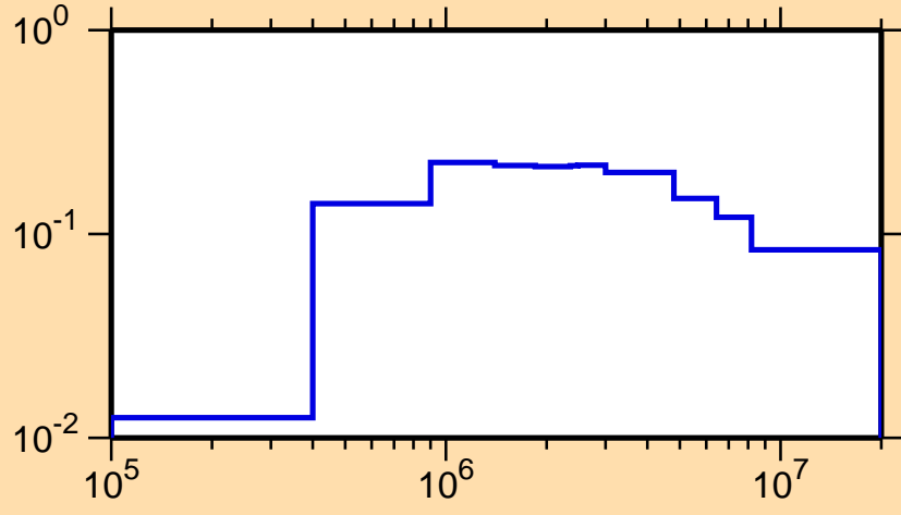
\sigma vs. E for ^{79}\text{Y}(n,\text{inel.})
