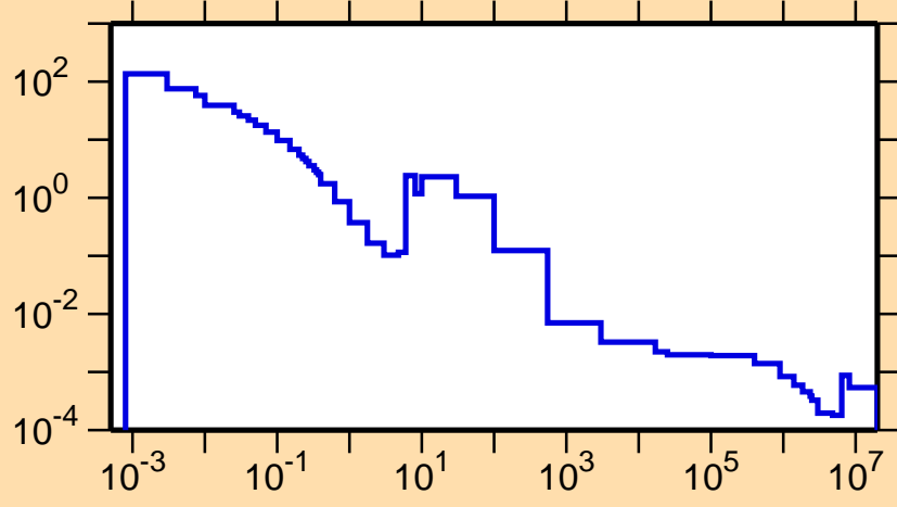
\sigma vs. E for ^{79}\text{Y}(n,\gamma)
