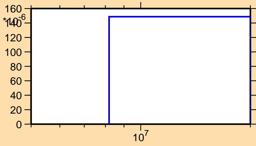
\sigma vs. E for ^{79}\text{Y}(n,t)
