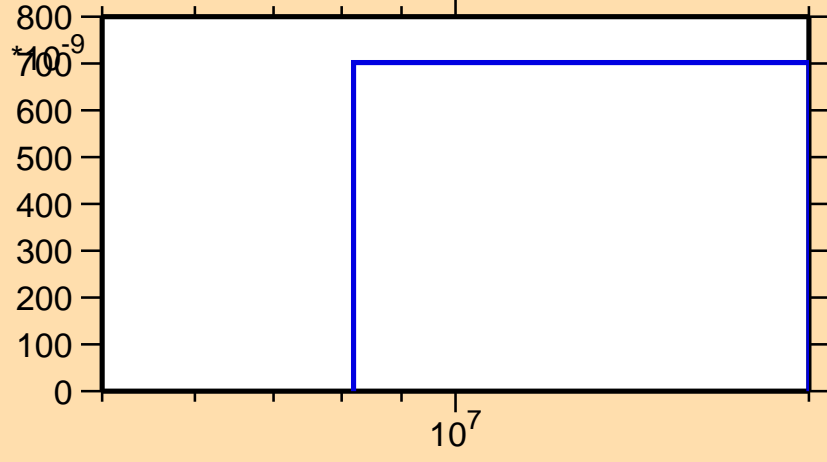
\sigma vs. E for ^{79}\text{Y} (mt 45)
