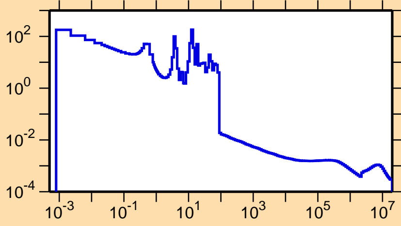
\sigma vs. E for ^{80}\text{Y}(n,\gamma)
