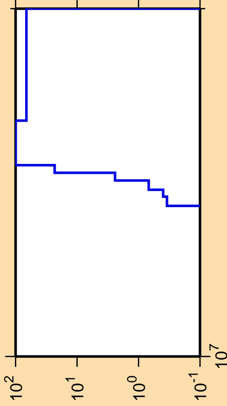
\Delta\sigma/\sigma vs. E for ^{80}\text{Y}(n,2np)
