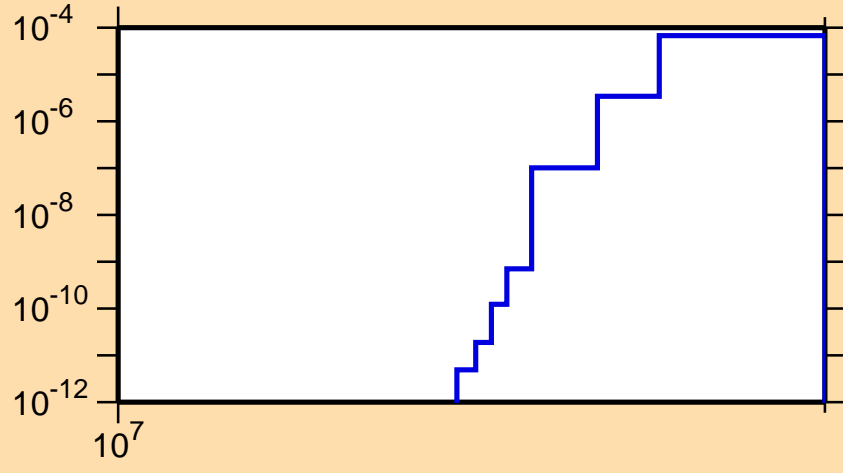
\sigma vs. E for ^{80}\text{Y}(n,\text{pt})
