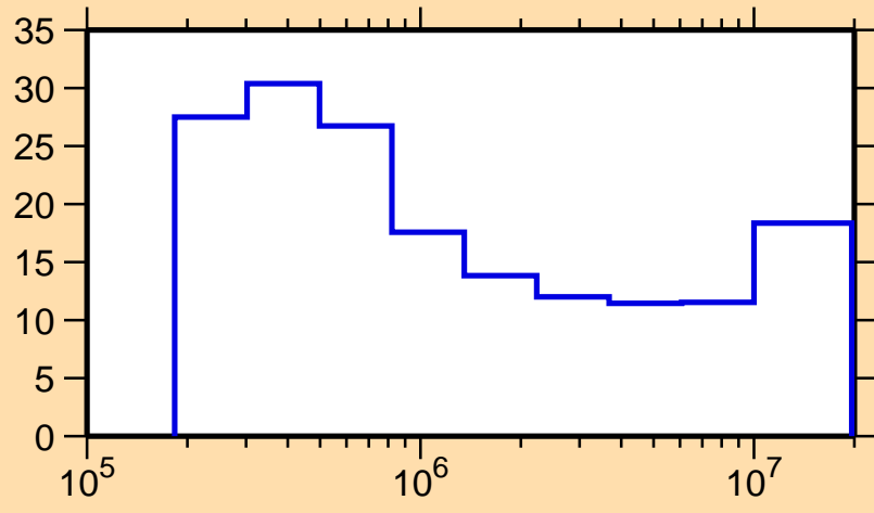
\Delta\sigma/\sigma vs. E for ^{80}\text{Y}(n,\text{tot.})
