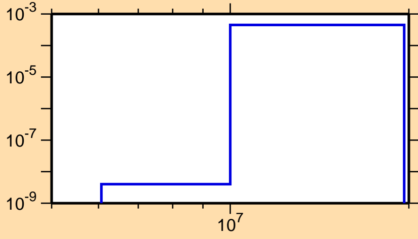
\sigma vs. E for ^{80}\text{Y}(n,n\alpha)
