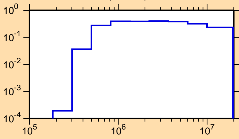
\sigma vs. E for ^{80}\text{Y}(n,\text{inel.})
