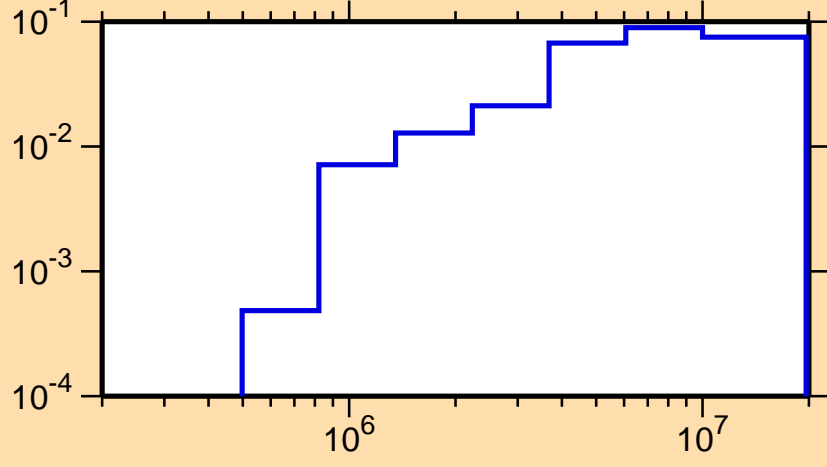
\sigma vs. E for ^{80}\text{Y}(n,n\text{cont.})
