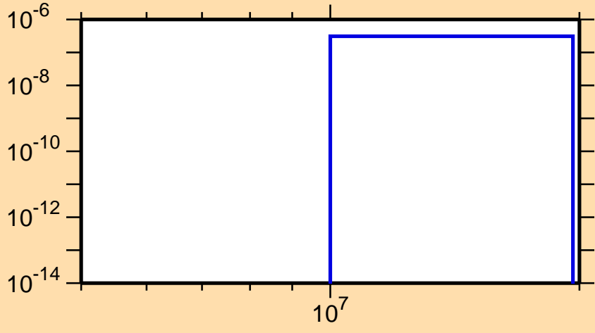
\sigma vs. E for ^{80}\text{Y} (mt 45)
