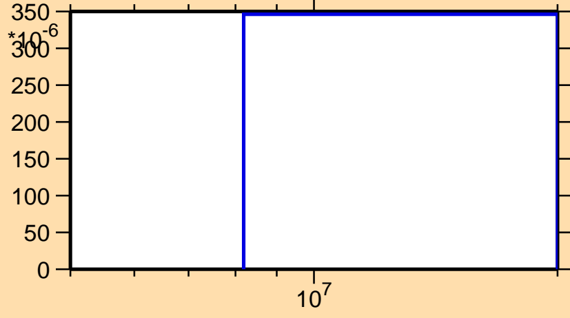
\sigma vs. E for ^{80}\text{Y}(n,2n)
