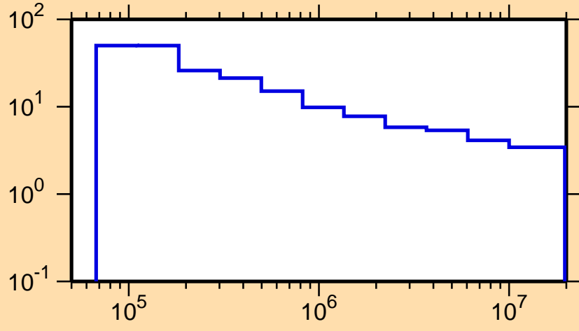
\Delta\sigma/\sigma vs. E for ^{80}\text{Y}(n,n\text{onel.})
