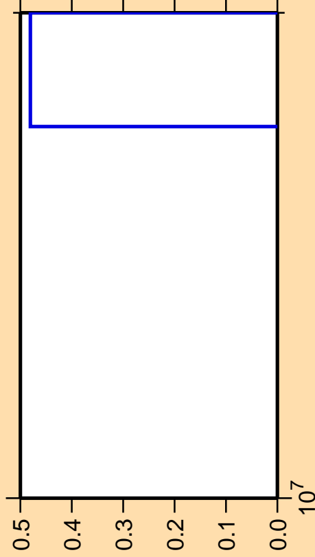
\Delta\sigma/\sigma vs. E for ^{81}\text{Y}(n,nt)
