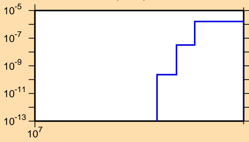
\sigma vs. E for ^{81}\text{Y}(n,nd)
