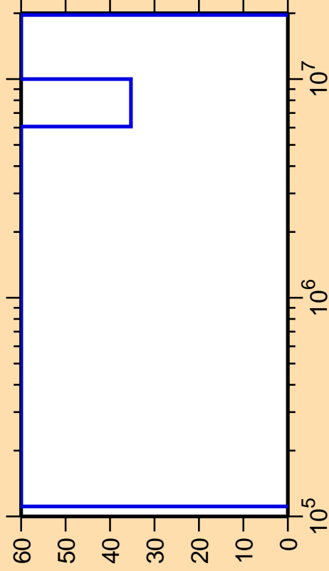
\Delta\sigma/\sigma vs. E for ^{81}\text{Y}(n,\gamma)
