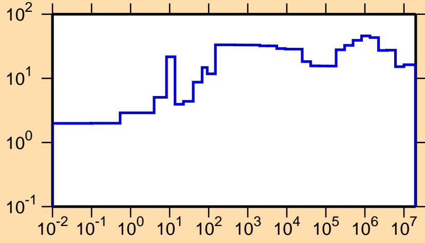
\Delta\sigma/\sigma vs. E for ^{81}\text{Y}(n,el.)
