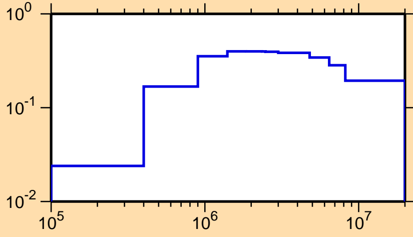
\sigma vs. E for ^{81}\text{Y}(n,\text{inel.})
