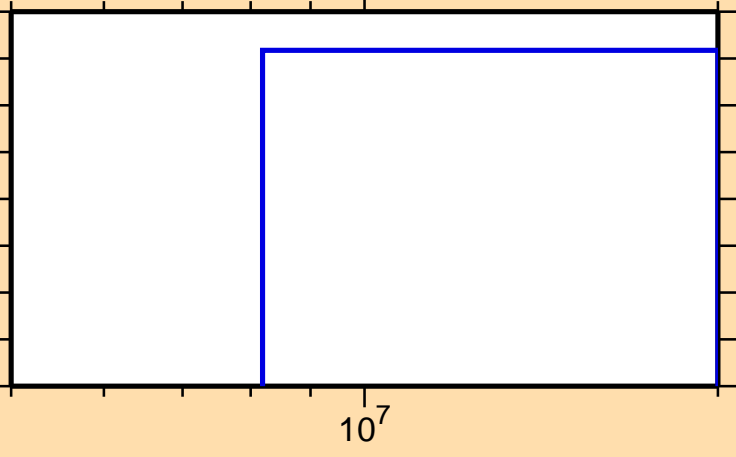
\sigma vs. E for ^{81}\text{Y}(n,\text{nd})
