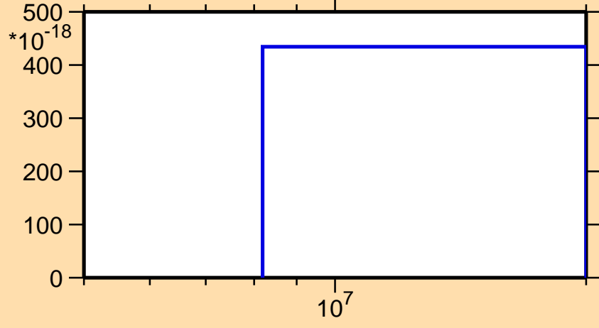
\sigma vs. E for ^{81}\text{Y}(n,nt)
