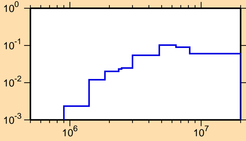
\sigma vs. E for ^{81}\text{Y}(n,n\text{cont.})
