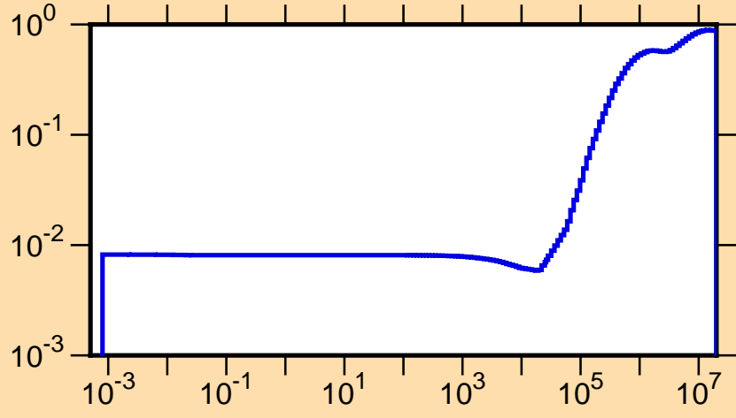
\mu vs. E for ^{82}\text{Y}(\text{mt251})
