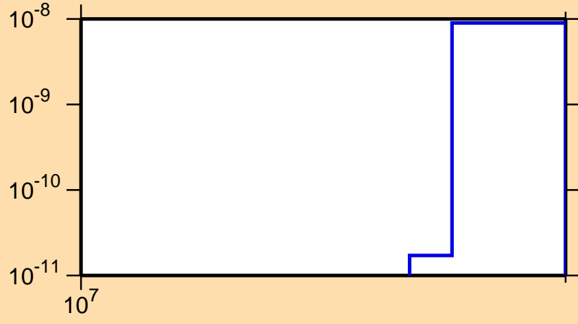
\sigma vs. E for ^{82}\text{Y} (mt 34)
