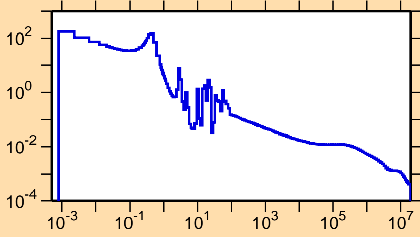
\sigma vs. E for ^{82}\text{Y}(n,\gamma)
