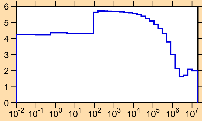
\sigma vs. E for ^{82}\text{Y}(n,\text{el.})
