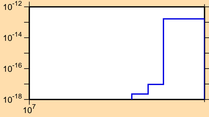
\sigma vs. E for ^{83}\text{Y} (mt 34)
