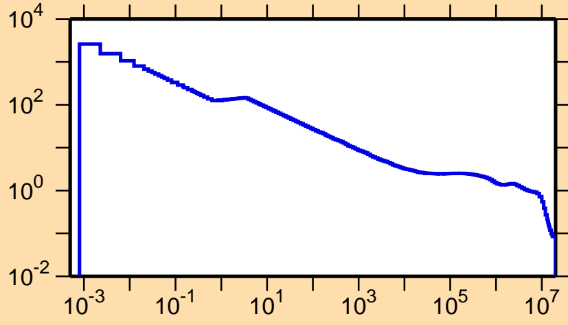
\sigma vs. E for ^{83}\text{Y}(n,p)
