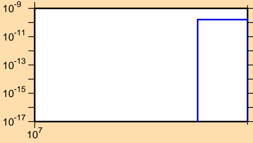
\sigma vs. E for ^{83}\text{Y}(n,\text{pt})
