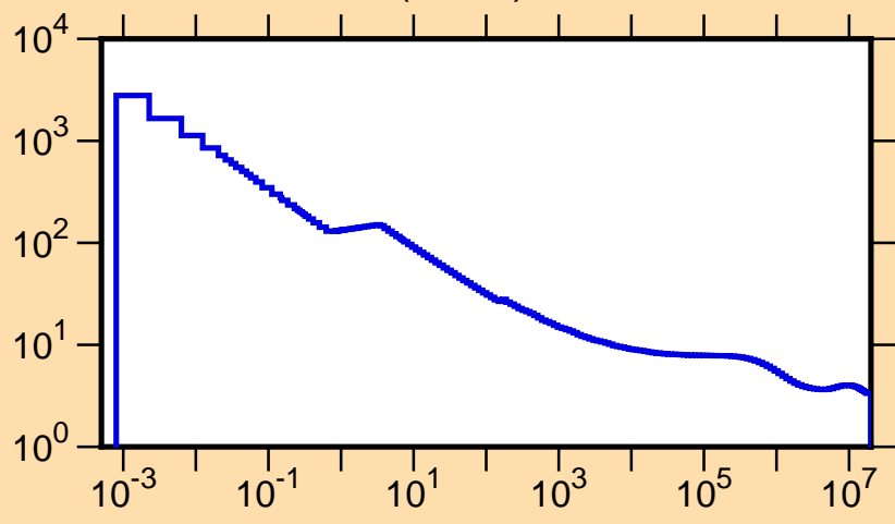
\sigma vs. E for ^{83}\text{Y}(n,\text{tot.})
