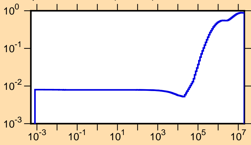
\mu vs. E for ^{84}\text{Y}(\text{mt251})
