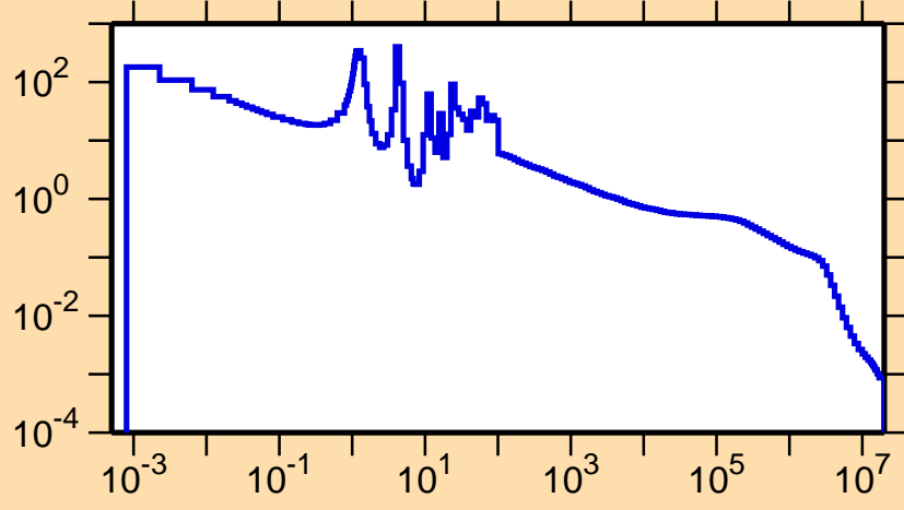
\sigma vs. E for ^{84}\text{Y}(n,\gamma)
