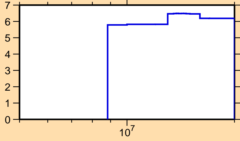
\Delta\sigma/\sigma vs. E for ^{84}\text{Y}(n,\text{nonel.})
