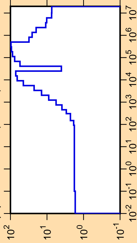
\Delta\mu/\mu vs. E for ^{84}\text{Y}(\text{mt251})
