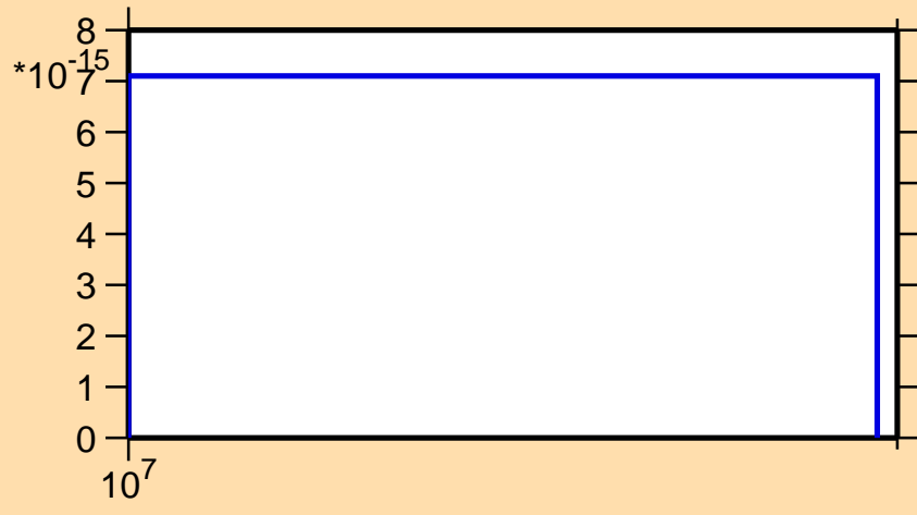
\sigma vs. E for ^{84}\text{Y}(n,nt)
