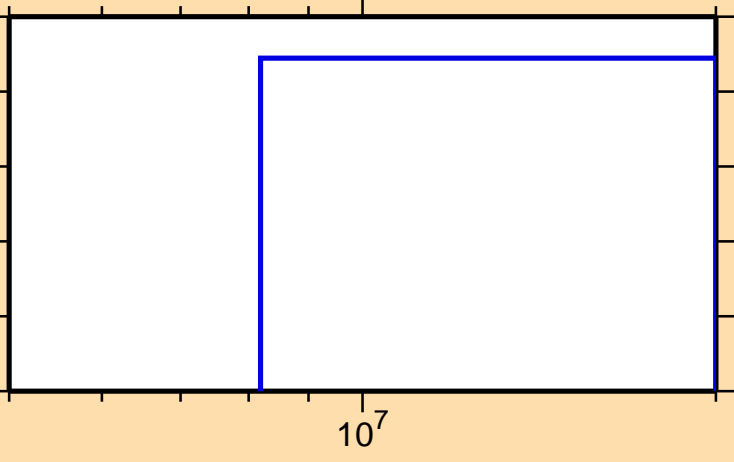
\sigma vs. E for ^{84}\text{Y}(n,\text{nd})
