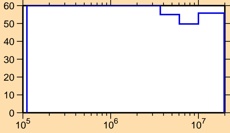
\Delta\sigma/\sigma vs. E for ^{84}\text{Y}(n,n\text{cont.})
