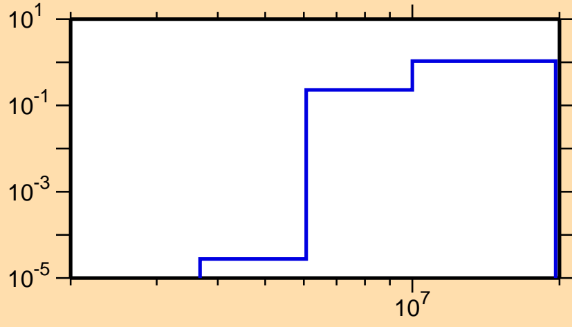
\sigma vs. E for ^{84}\text{Y}(n,np)
