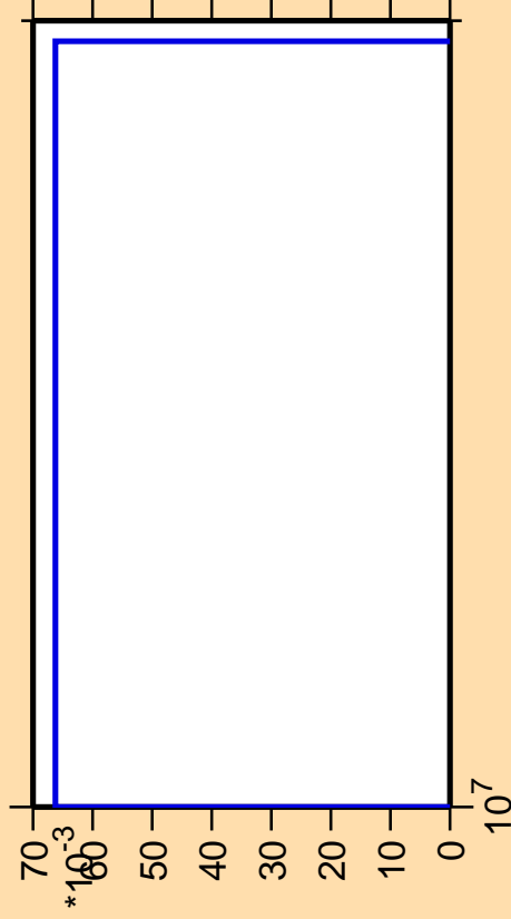
\Delta\sigma/\sigma vs. E for ^{84}\text{Y}(n,nt)
