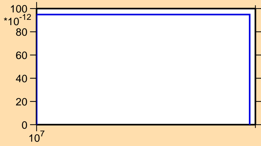
\sigma vs. E for ^{84}\text{Y}(\text{mt117})
