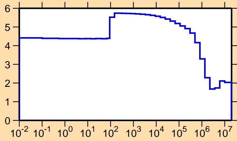
\sigma vs. E for ^{84}\text{Y}(n,\text{el.})
