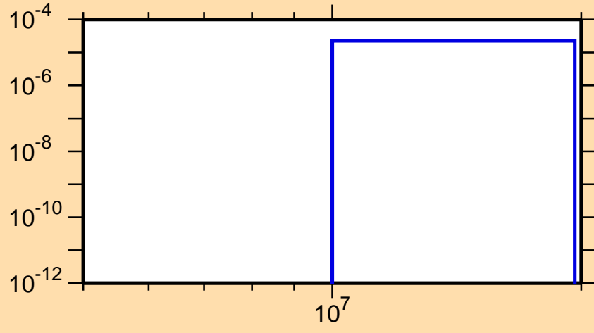
\sigma vs. E for ^{84}\text{Y}(n,\text{He}3)
