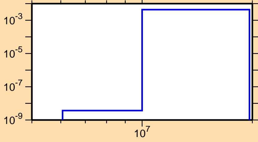
\sigma vs. E for ^{84}\text{Y}(n,n\alpha)
