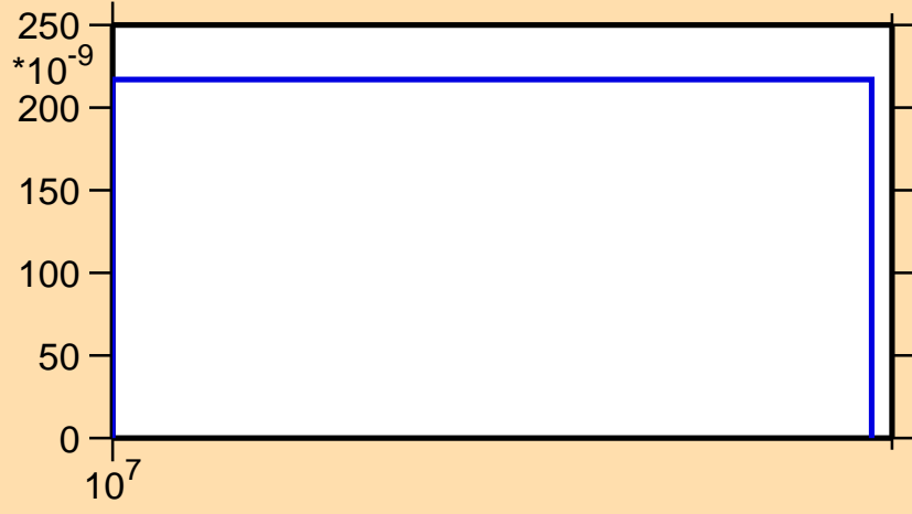
\sigma vs. E for ^{84}\text{Y}(n,\text{pd})
