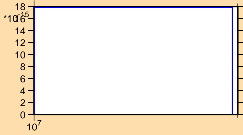
\sigma vs. E for ^{84}\text{Y}(n,nt)
