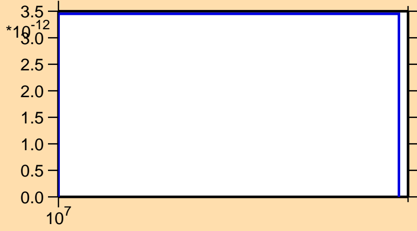
\sigma vs. E for ^{84}\text{Y} (mt 34)
