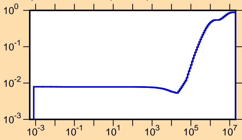
\mu vs. E for ^{85}\text{Y}(\text{mt251})
