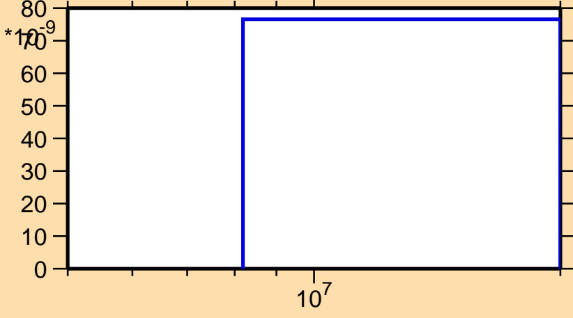
\sigma vs. E for ^{85}\text{Y}(n,\text{nd})
