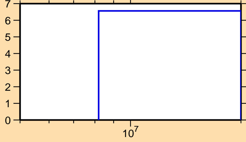
\Delta\sigma/\sigma vs. E for ^{85}\text{Y}(n,\text{nonel.})
