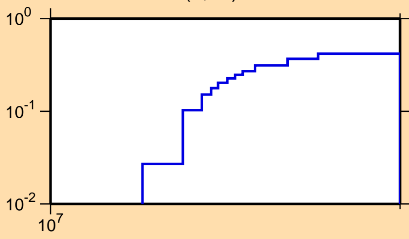
\sigma vs. E for ^{85}\text{Y}(n,2n)
