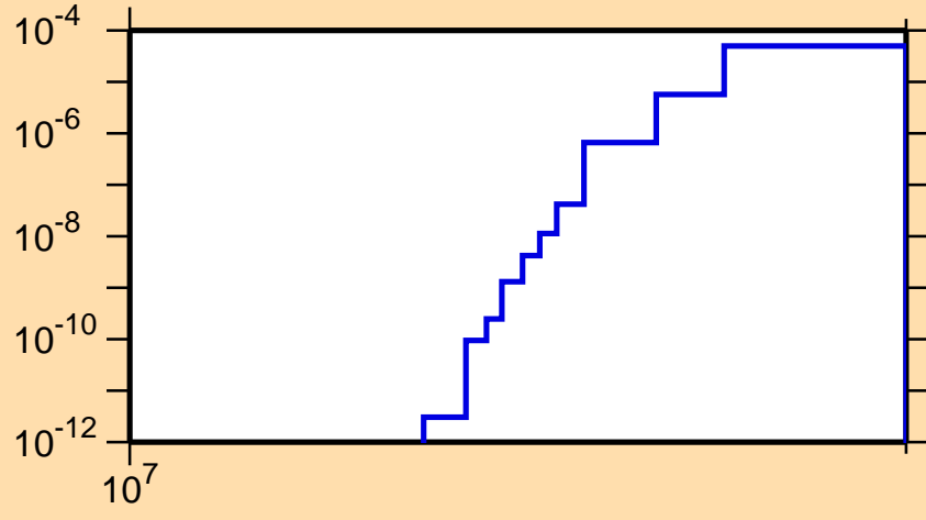
\sigma vs. E for ^{86}\text{Y}(n,nd)
