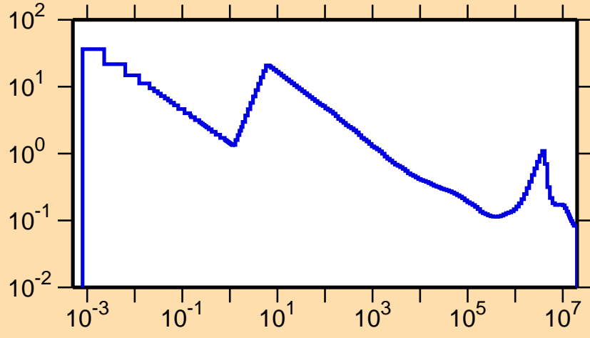
\sigma vs. E for ^{86}\text{Y}(n,p)
