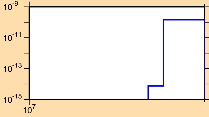
\sigma vs. E for ^{86}\text{Y} (mt 45)
