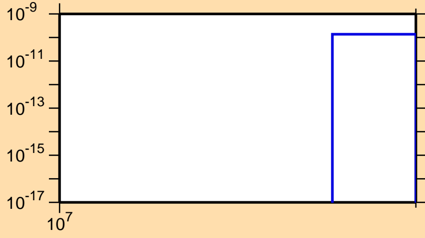
\sigma vs. E for ^{86}\text{Y}(n,2n\alpha)
