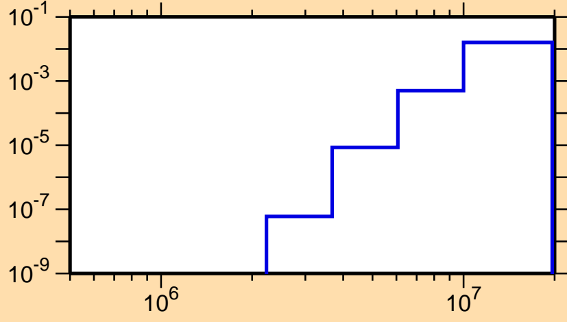
\sigma vs. E for ^{87}\text{Y}(n,\alpha)
