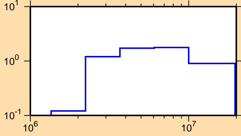
\sigma vs. E for ^{87}\text{Y}(n,n\text{cont.})
