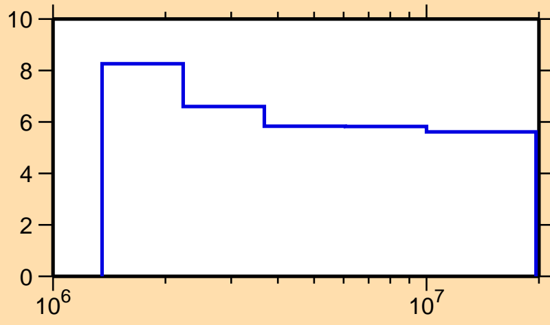
\Delta\sigma/\sigma vs. E for ^{87}\text{Y}(n,n\text{onel.})
