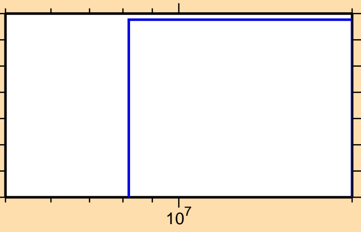
\sigma vs. E for ^{87}\text{Y}(\text{mt117})
