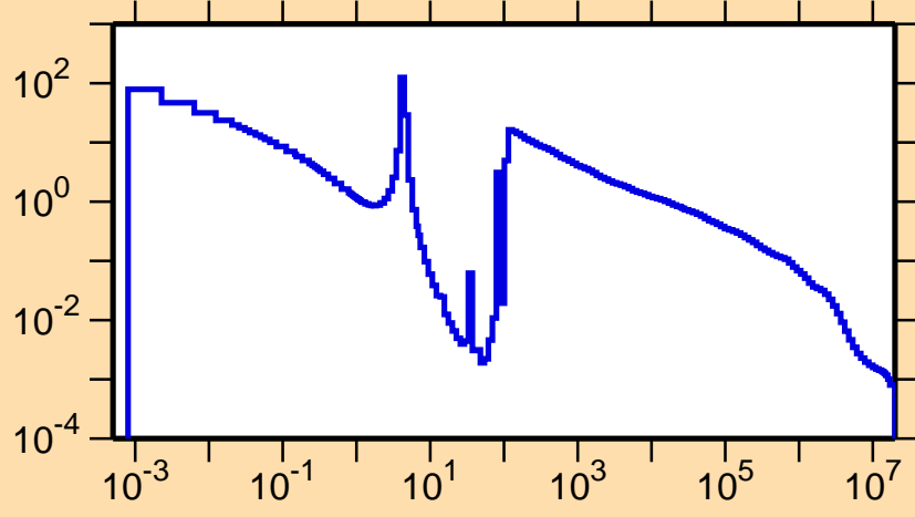
\sigma vs. E for ^{88}\text{Y}(n,\gamma)
