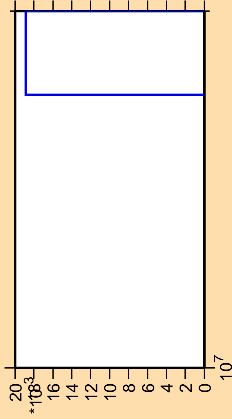
\Delta\sigma/\sigma vs. E for ^{88}\text{Y}(n,nt)
