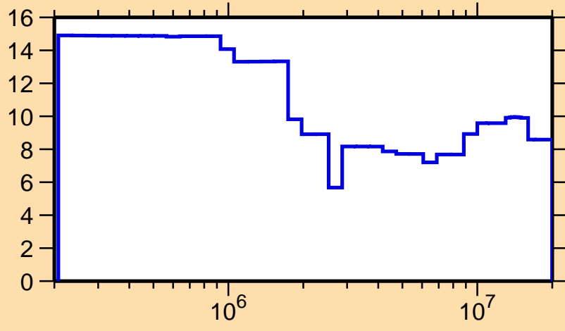
\Delta\sigma/\sigma vs. E for ^{88}\text{Y}(n,\text{el.})
