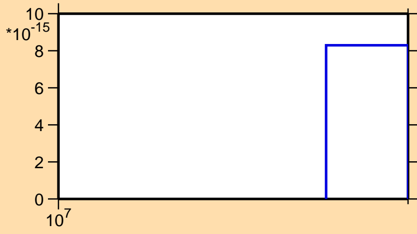
\sigma vs. E for ^{88}\text{Y}(n,nt)
