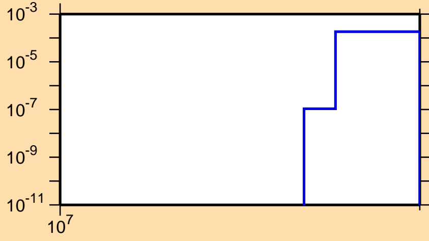
\sigma vs. E for ^{88}\text{Y}(n,2np)
