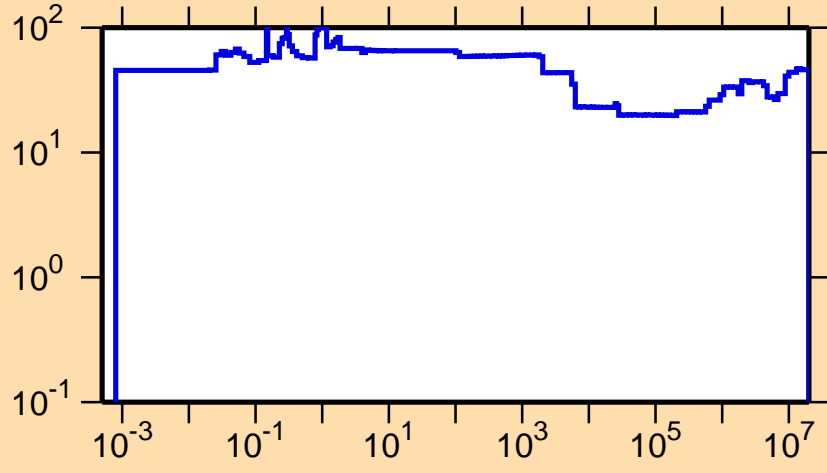
\Delta\sigma/\sigma vs. E for ^{88}\text{Y}(n,p)
