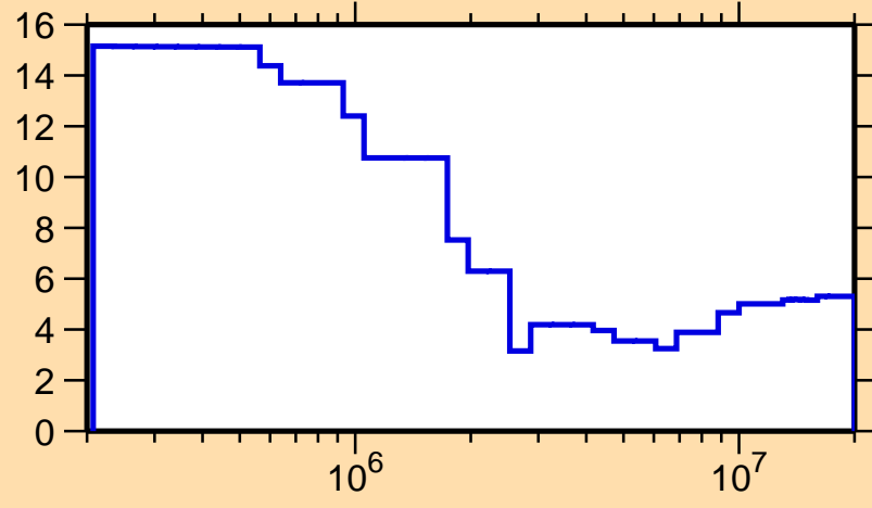
\Delta\sigma/\sigma vs. E for ^{88}\text{Y}(n,\text{tot.})
