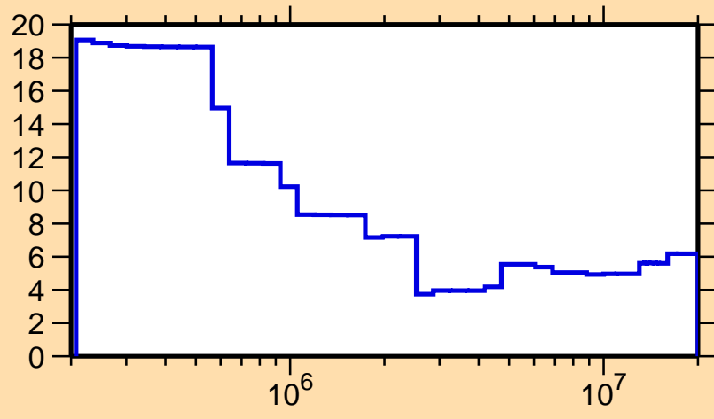
\Delta\sigma/\sigma vs. E for ^{88}\text{Y}(n,\text{nonel.})
