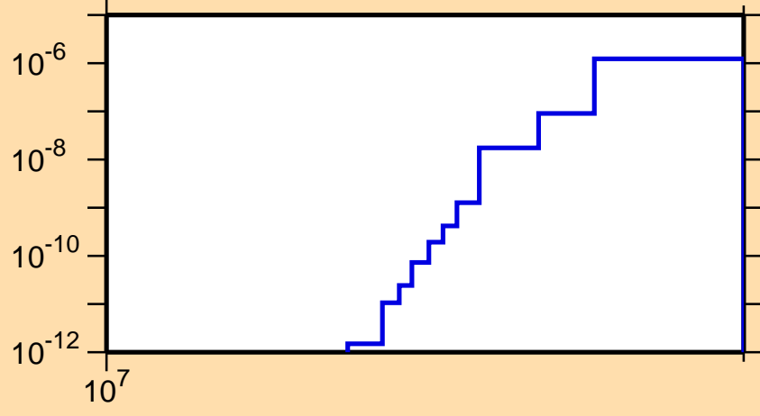
\sigma vs. E for ^{88}\text{Y}(n,\text{He}3)
