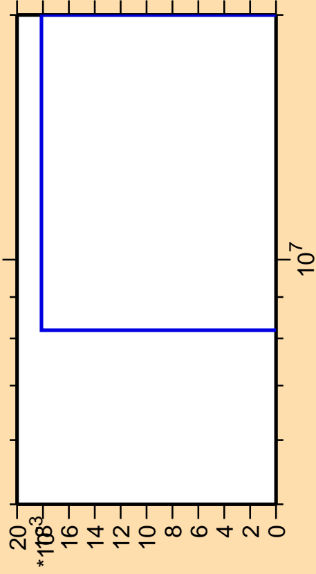
\Delta\sigma/\sigma vs. E for ^{88}\text{Y}(n,\text{pd})
