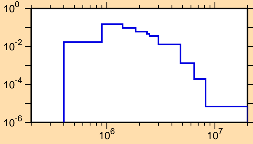
\sigma vs. E for ^{88}\text{Y}(n,n_4)
