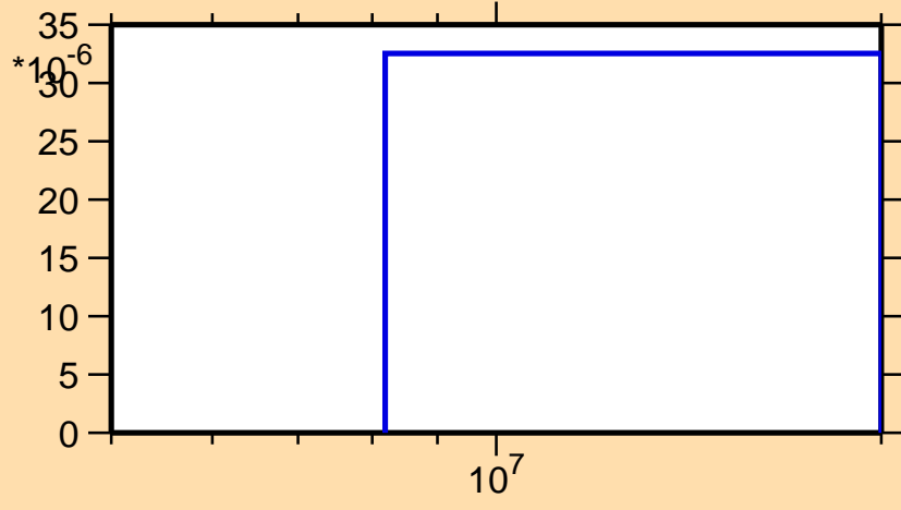
\sigma vs. E for ^{88}\text{Y}(n,n\alpha)
