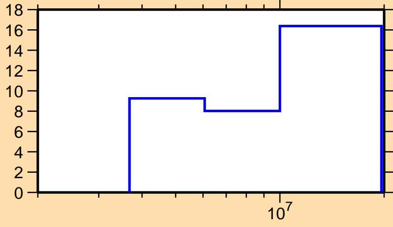
\Delta\sigma/\sigma vs. E for ^{89}\text{Y}(n,ncont.)
