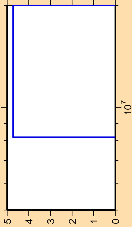
\Delta\sigma/\sigma vs. E for ^{89}\text{Y}(n,2np)
