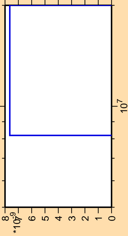
\Delta\sigma/\sigma vs. E for ^{89}\text{Y}(n,2n\alpha)
