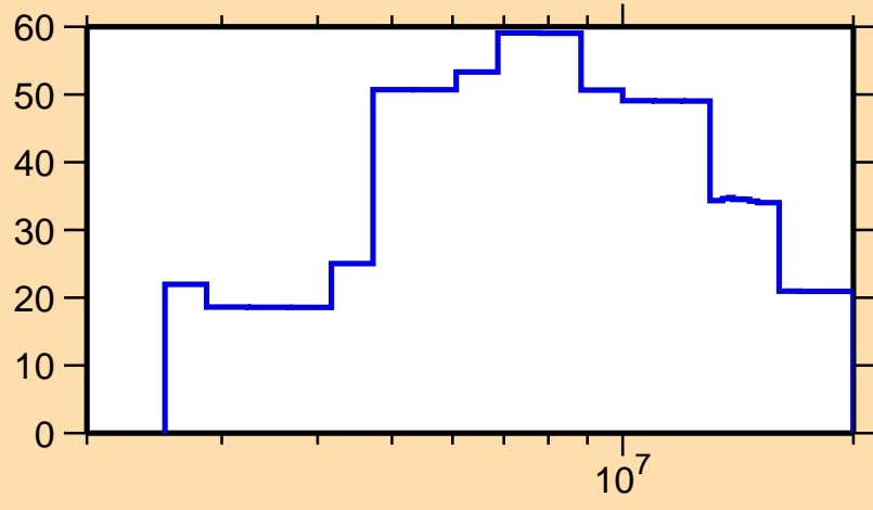
\Delta\sigma/\sigma vs. E for ^{89}\text{Y}(n,p)
