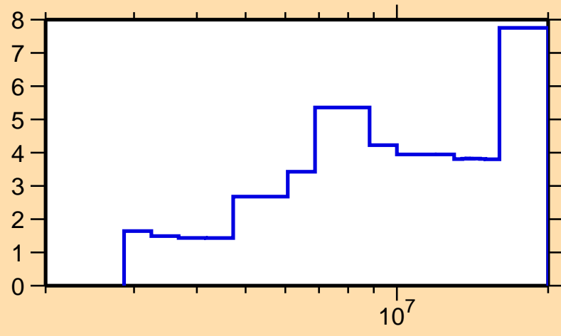
\Delta\sigma/\sigma vs. E for ^{89}\text{Y}(n,n\text{onel.})
