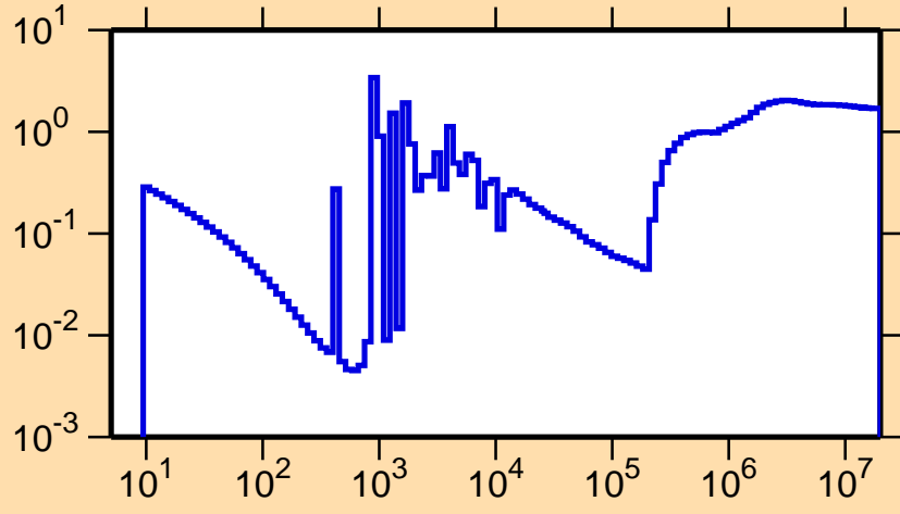
\sigma vs. E for ^{90}\text{Y}(n,\text{nonel.})
