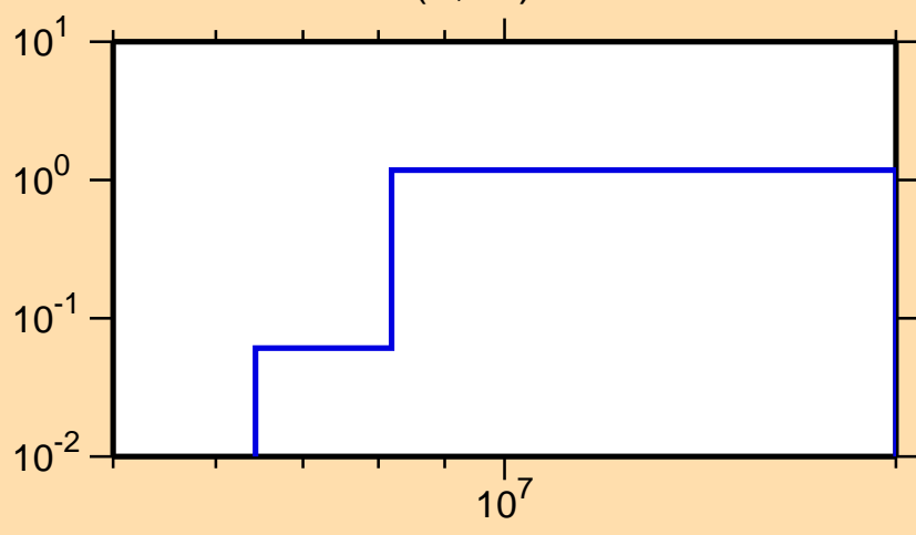
\sigma vs. E for ^{90}\text{Y}(n,2n)
