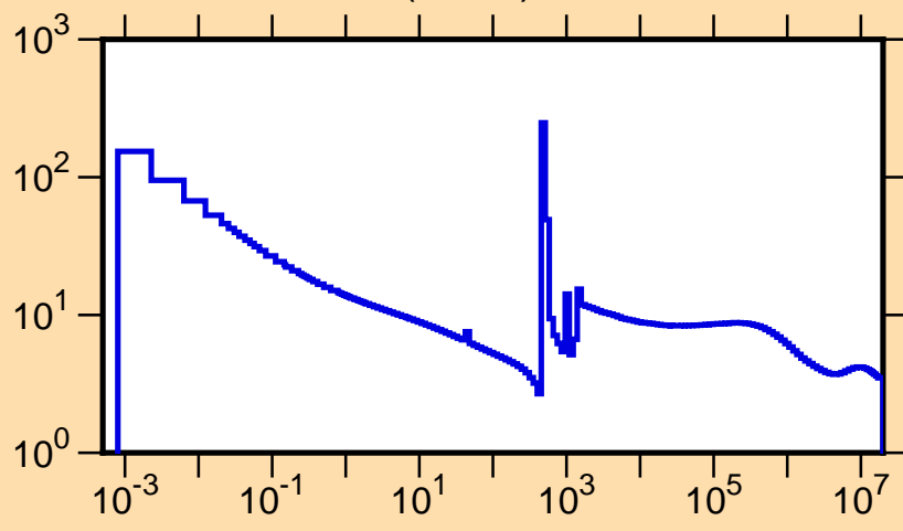
\sigma vs. E for ^{90}\text{Y}(n,\text{tot.})
