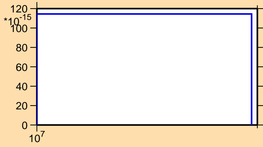
\sigma vs. E for ^{90}\text{Y}(n,2n\alpha)
