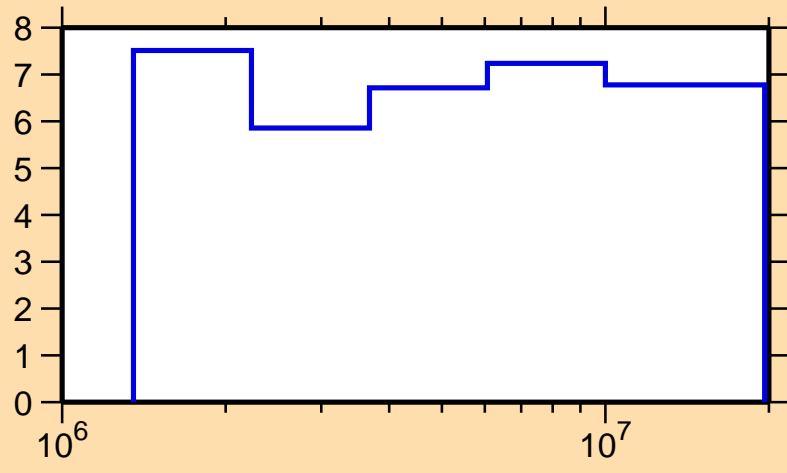
\Delta\sigma/\sigma vs. E for ^{90}\text{Y}(n,n\text{onel.})
