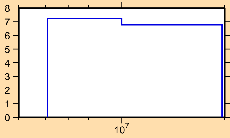
\Delta\sigma/\sigma vs. E for ^{90}\text{Y}(n,\text{nonel.})
