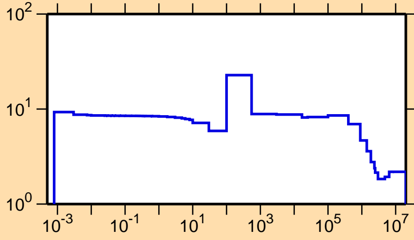
\sigma vs. E for ^{90}\text{Y}(n,\text{el.})
