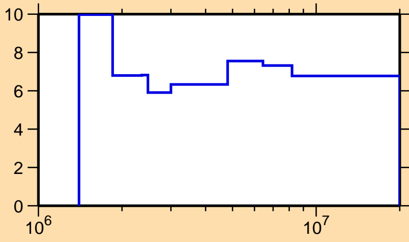
\Delta\sigma/\sigma vs. E for ^{90}\text{Y}(n,n\text{onel.})
