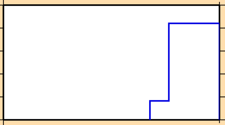
\sigma vs. E for ^{91}\text{Y}(n,\text{He}3)
