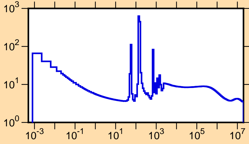
\sigma vs. E for ^{91}\text{Y}(n,\text{tot.})
