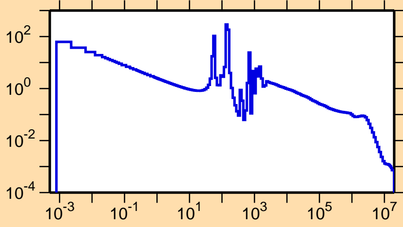
\sigma vs. E for ^{91}\text{Y}(n,\gamma)
